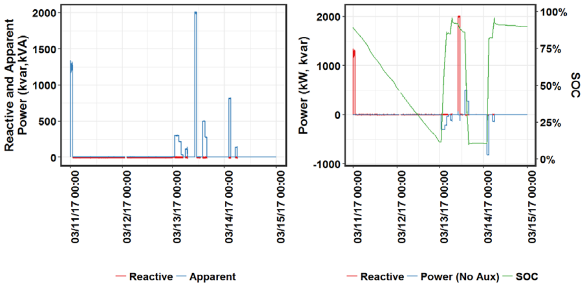
Figure 2.18. Power Factor Correction Mode, Run 1, Cycle 2 (left) Reactive Power and total kVA, (right) Real and Reacive Power, SOC. Reactive power not being requested when real power flows.
