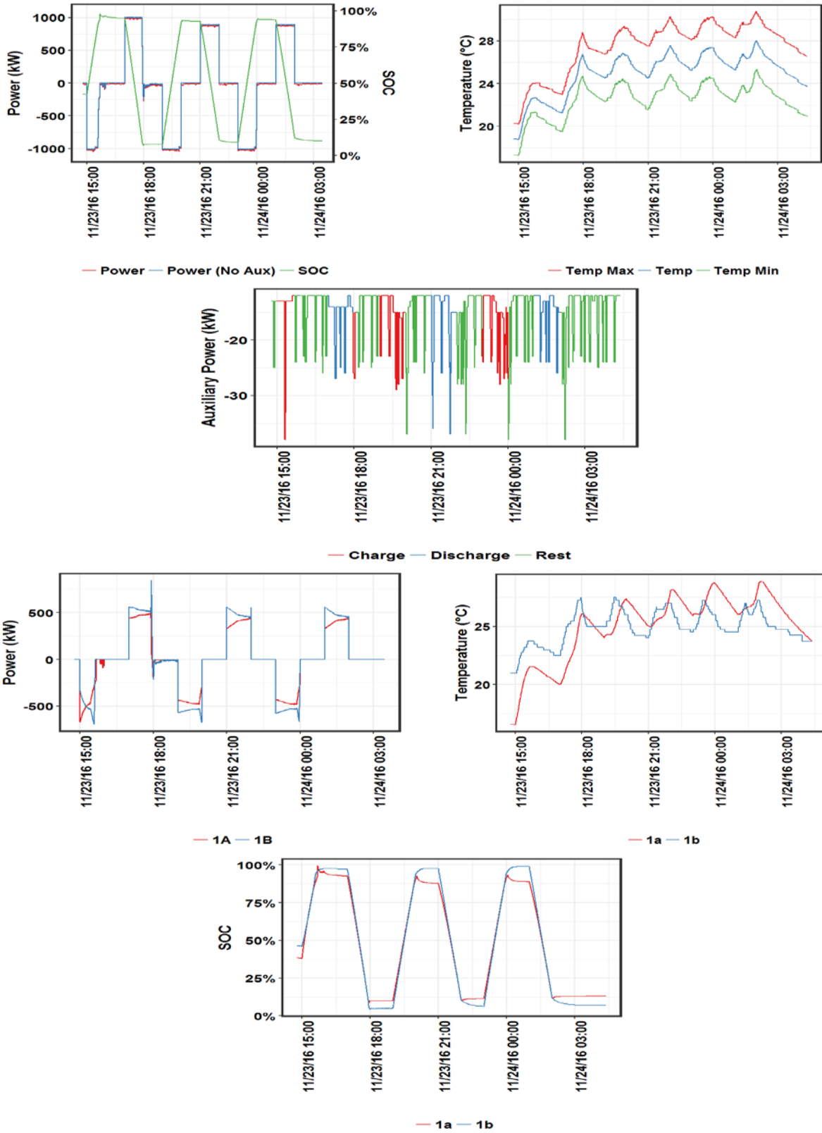
Figure 2.28. Power, SOC, Temperature and Auxiliary Consumption for Capacity Tests Post Cycle 1 at C Rate; (top) BESS, (bottom) MESA-11a and 1b
