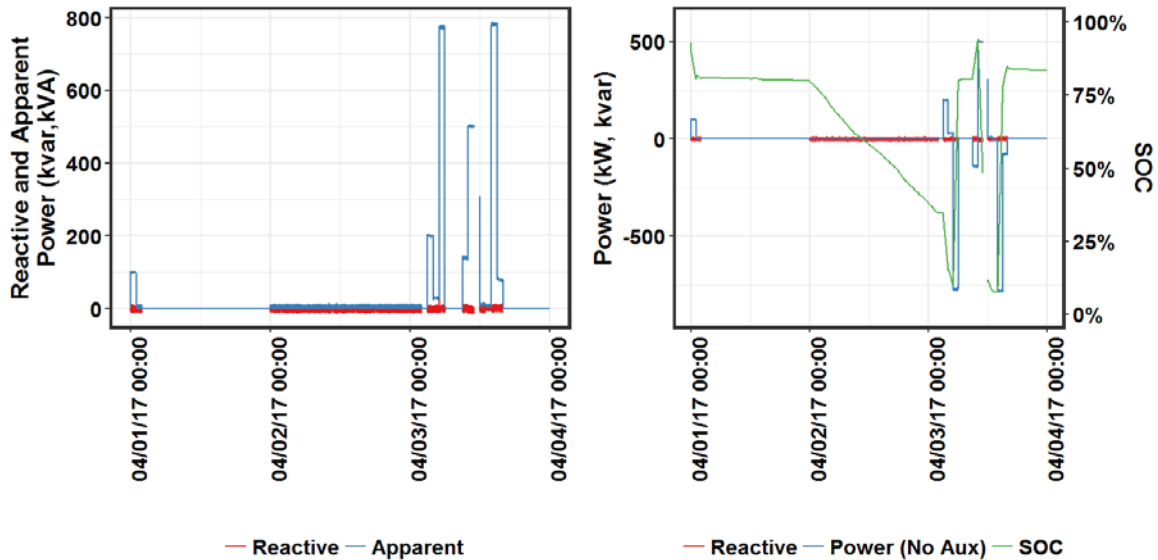
Figure 2.19. Power Factor Correction Mode, Run 2, Cycle 2 (left) Reactive Power and Total kVA, (right) Real and Reacive Power, SOC. Negligible reactive power flow.
