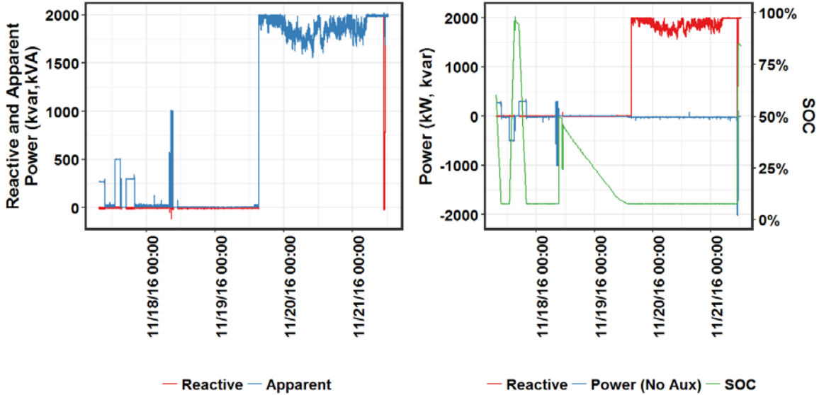
Figure 2.17. Power Factor Correction Mode, Run 3, Cycle 1 (left) Reactive Power and Total kVA, (right) Real and Reacive Power, SOC. The duty cycle starts 8 AM 11/19/16.
