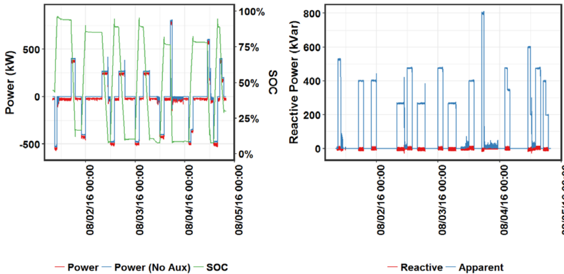
Figure 2.21. PCS Switching State as a Function of SOC Level after Discharge (left) Real Power, (right) Apparent and Reactive Power
