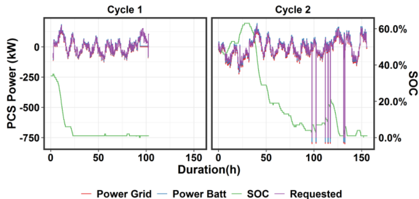
Figure 2.17. Load Shaping Test
