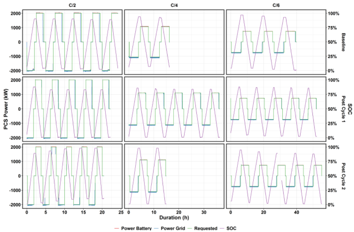
Figure 2.3. Power and SOC Profiles for BESS at C/2, C/4, and C/6 rates for Reference Performance Capacity Baseline, Post Cycle 1 and Post Cycle 2 Tests
