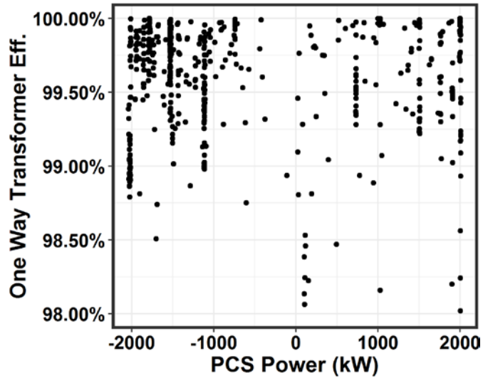
Figure 1.8. One-Way 480 VAC to 12 kVAC Transformer Efficiency
