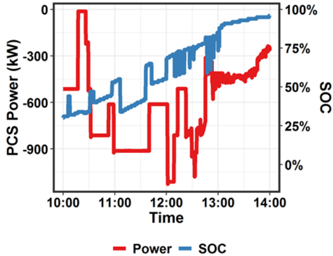
Figure 1.3. SOC Change with Rapid Power Swings
