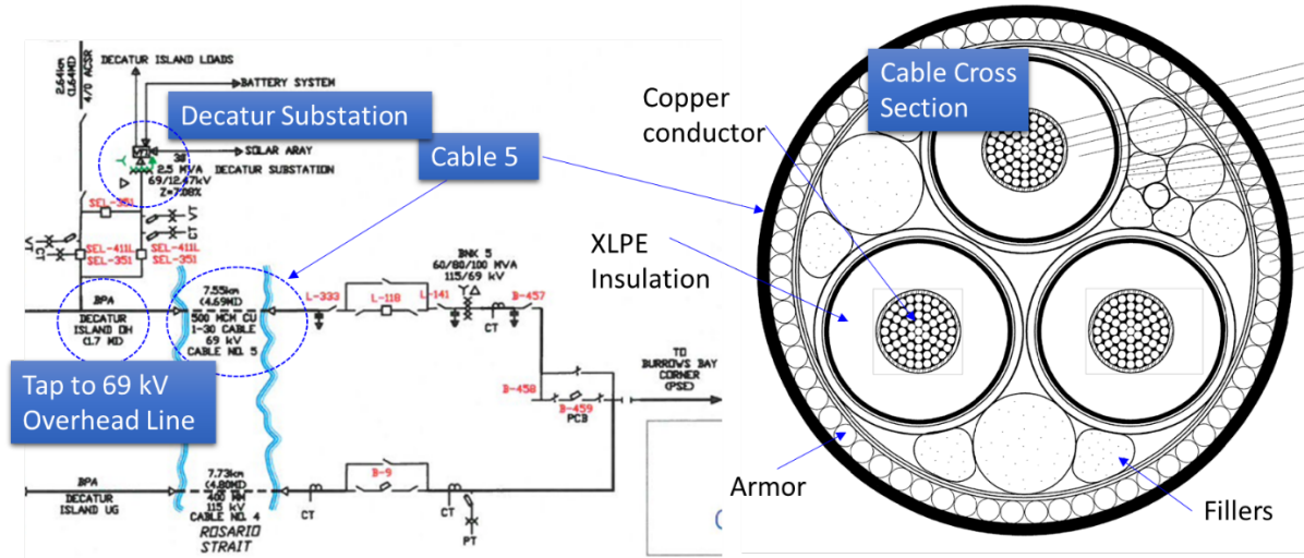
Figure 2.2. Cable 5 and ESS site at Decatur Substation in the OPALCO Single Line Diagram (left); Cable 5 Cross Section (right)
