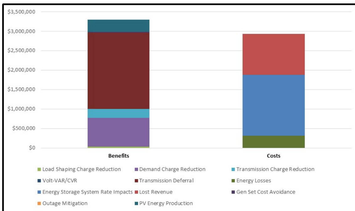
Figure ES.2. Base Case Benefits and Costs for the Decatur Island Community Solar and Energy Storage Project
