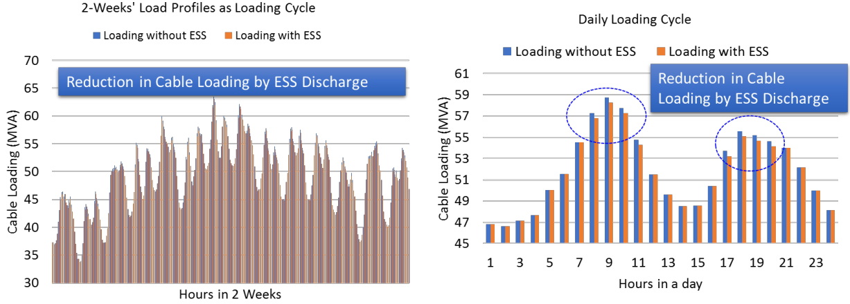
Figure 2.4. Two-Weeks Load Profile as Loading Cycle (left); Daily Load Profile Showing Reduction in Loading Due to ESS Discharge (right)
