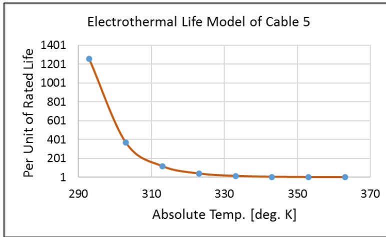
Figure 2.3. Electrothermal Life Model of Cable 5
